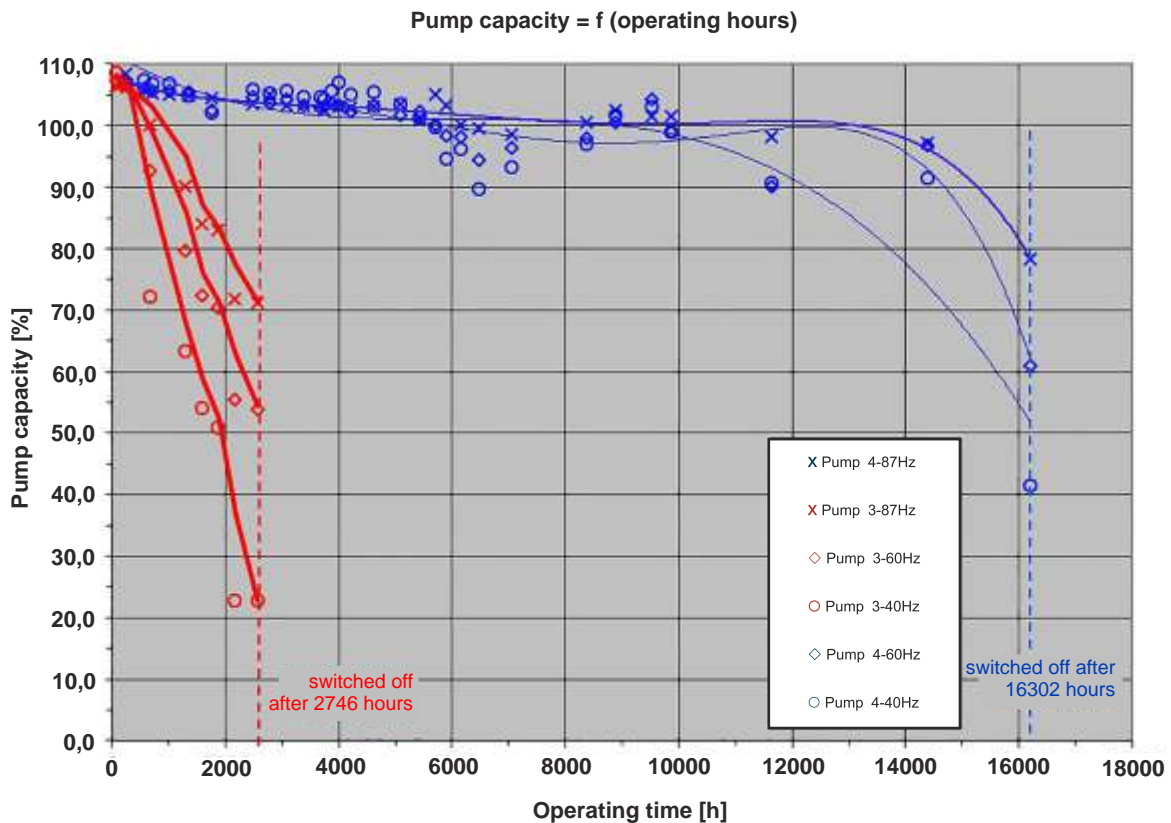
Comparative pumps of the AE4H750 series
